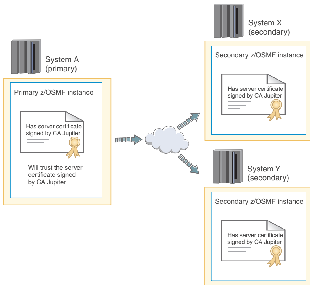
Figure 27. Trust relationship when server certificates are signed by the same CA certificate
