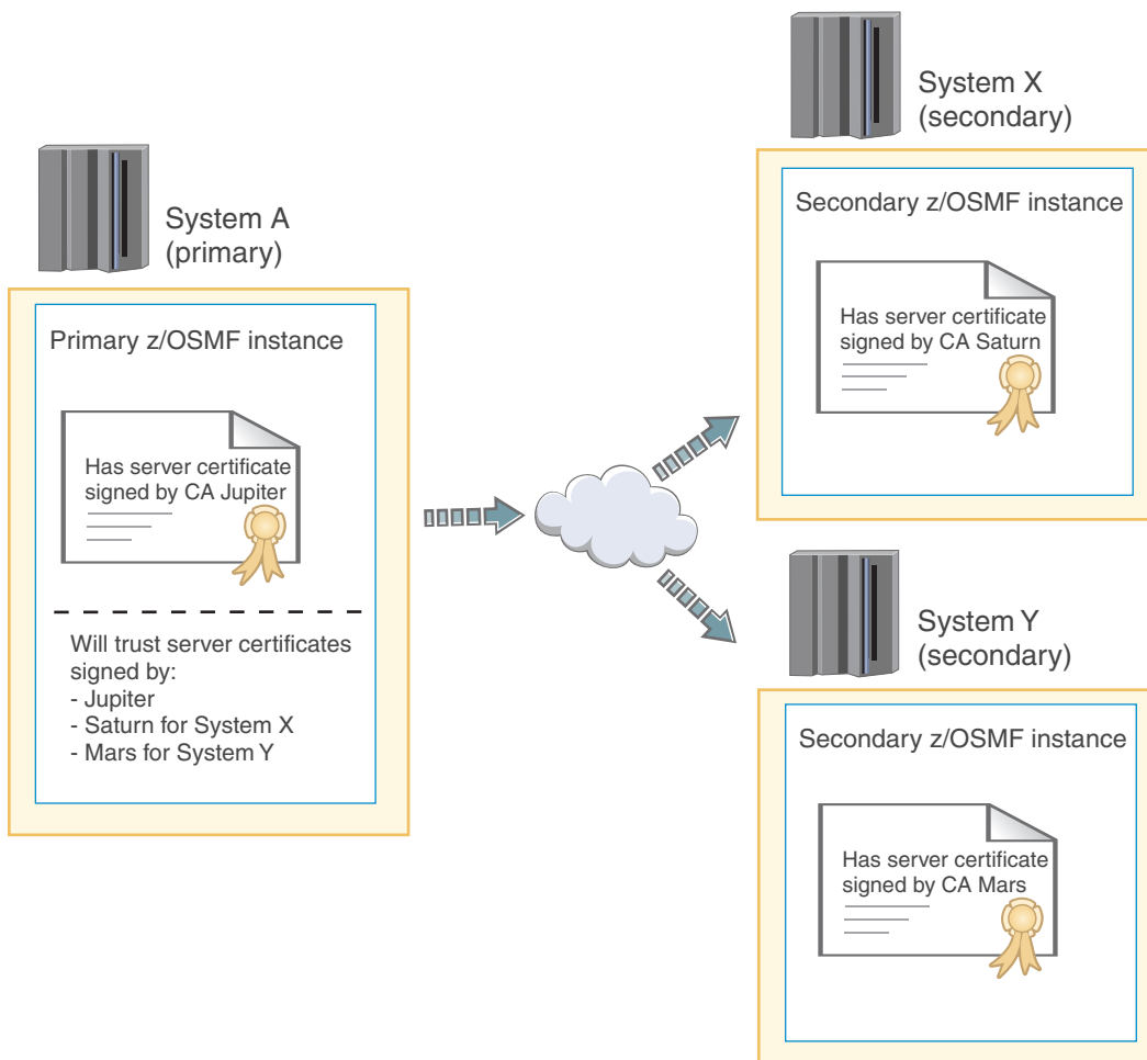
Figure 28. Trust relationship when the server certificates are signed by different CA certificates
