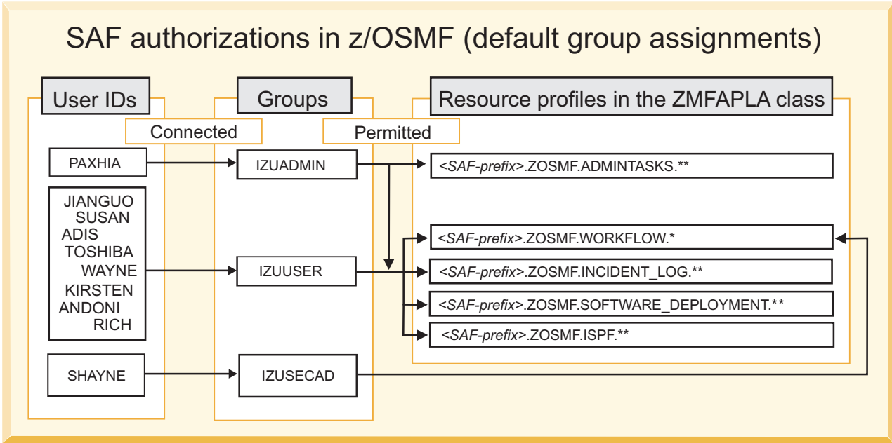
Figure 21. SAF authorizations in z/OSMF: The default setup
